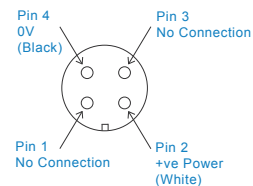
Connection Details
