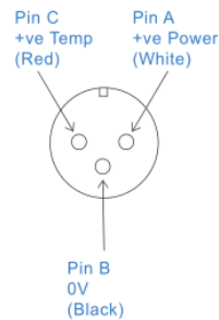
Connection Details
