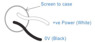
Connection Details
