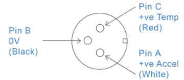
Connection Details
