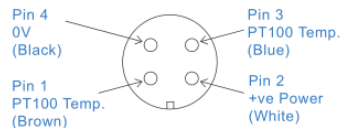
Connection Details
