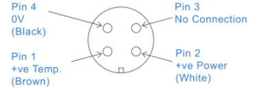
Connection Details
